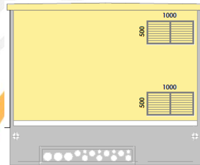
FAÇADE ARRIERE
